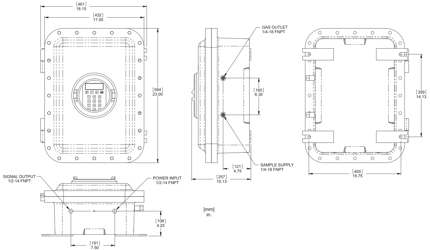
SS500/SS2000 Explosion Proof analyzer outline and mounting dimensions.
